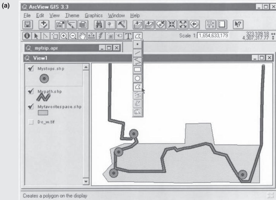
FIGURE 8.8 ArcView digitizing. (a) With the image feature turned off, the display shows point, line, and polygon features and the pull-down tool selections from which the appropriate tool was selected to accomplish the digitizing. (b) With the image feature turned on, the graphic shows what the display looks like after a student digitizes point, line, and polygon features.
